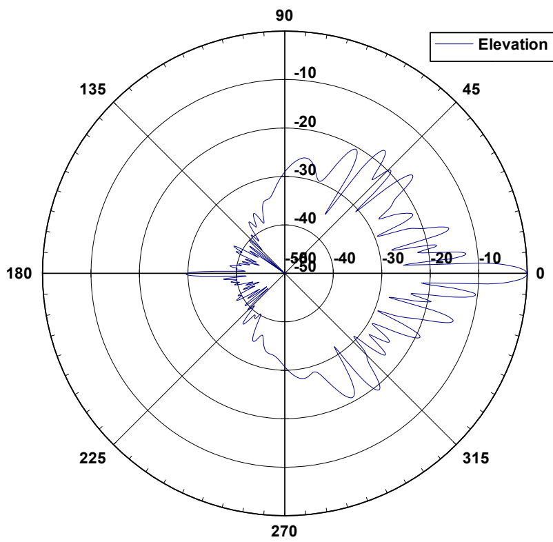
58 9004 Elevation Pattern
